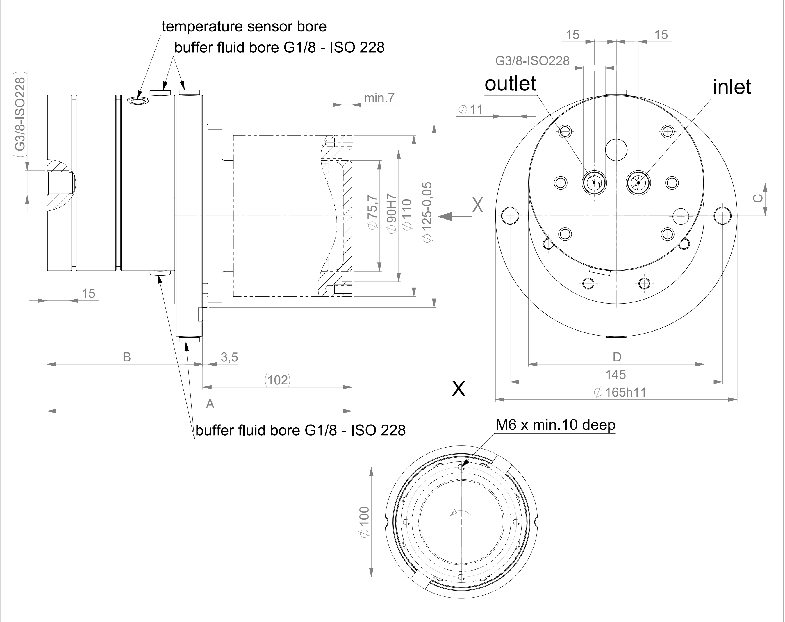
Assembly dimensions
