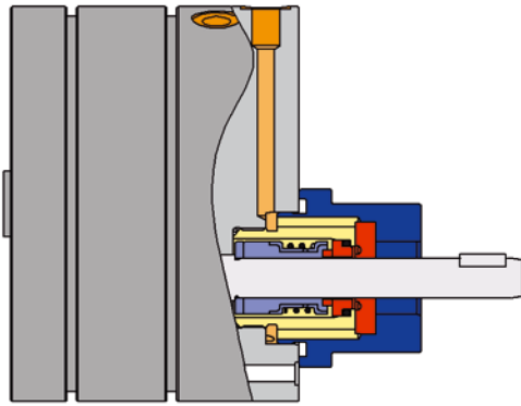
Mechanical seal
