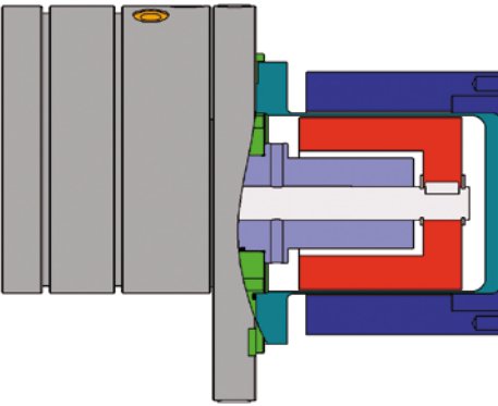
Magnetic coupling
