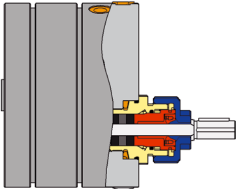
Stuffing box
